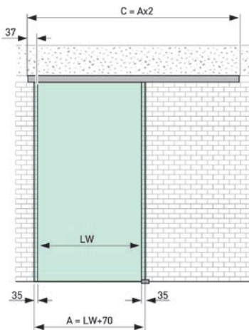
Systems with one sash with sidelight
