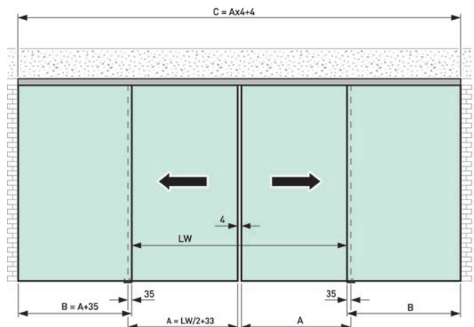
Systems with two sashes with sidelight
