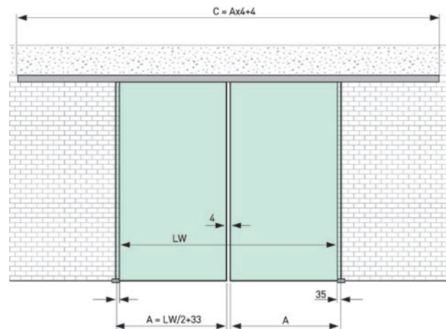
Systems with two sashes with sidelight
