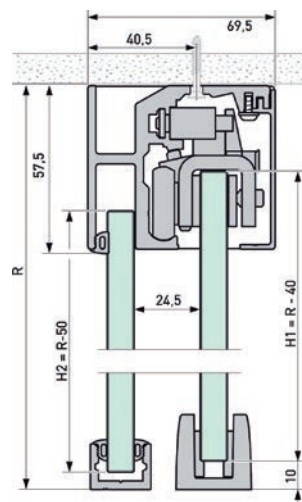
Ceiling-mounted track with sidelight
