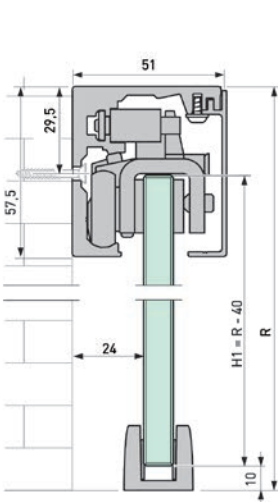
Systems with one sash without sidelight
